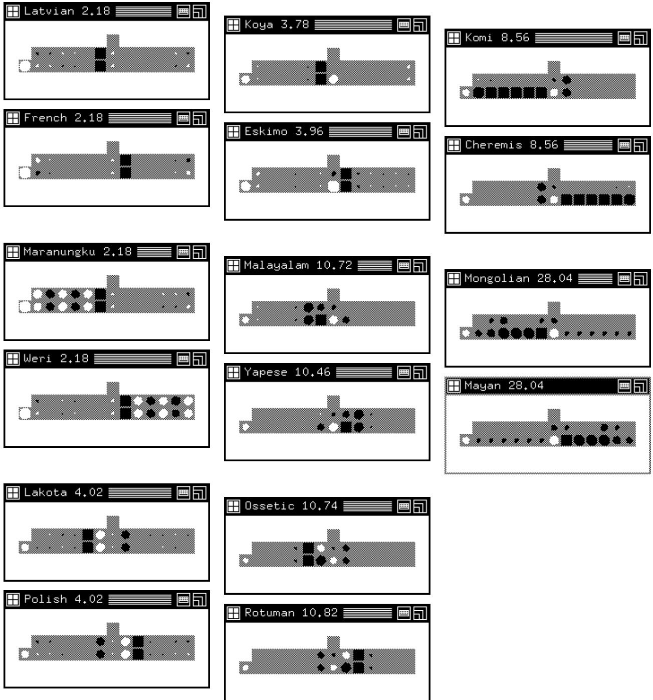
Figure 4: Learned connection weights for sixteen stress patterns. Each display is a representation of the network as a whole. The large grey shaded rectangle represents the input buffer of the network, organized as two rows of 13 values. The single square protruding from the left is the perceptron's bias connection. The perceptron unit itself is represented by the single protruding square at the top. A blob in a particular position denotes a weight from the unit in that position to the output unit. White blobs denote positive weights, and black blobs negative weights. The area of the blobs is proportional to the absolute magnitude of the weight. Weights are scaled so that the largest absolute magnitude is depicted in each display as a perfect square; other weights in that display appear as blobs of proportionate size. The scale is shown in the title bar of each display. Thus, for Maranungku, the absolute magnitude of the largest weights is 2.18; these are the large (black) negative weights left of center in the input layer.
