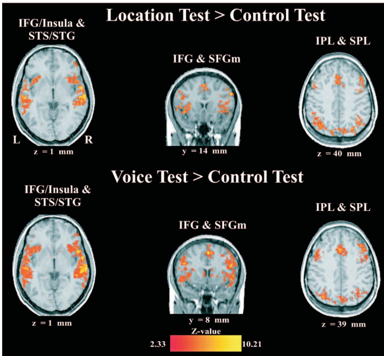
Figure 4. Cross-subject average statistical maps of activation during the test period of the location and voice tasks (relative to control task) overlaid on a Talairach normalized anatomical image.
